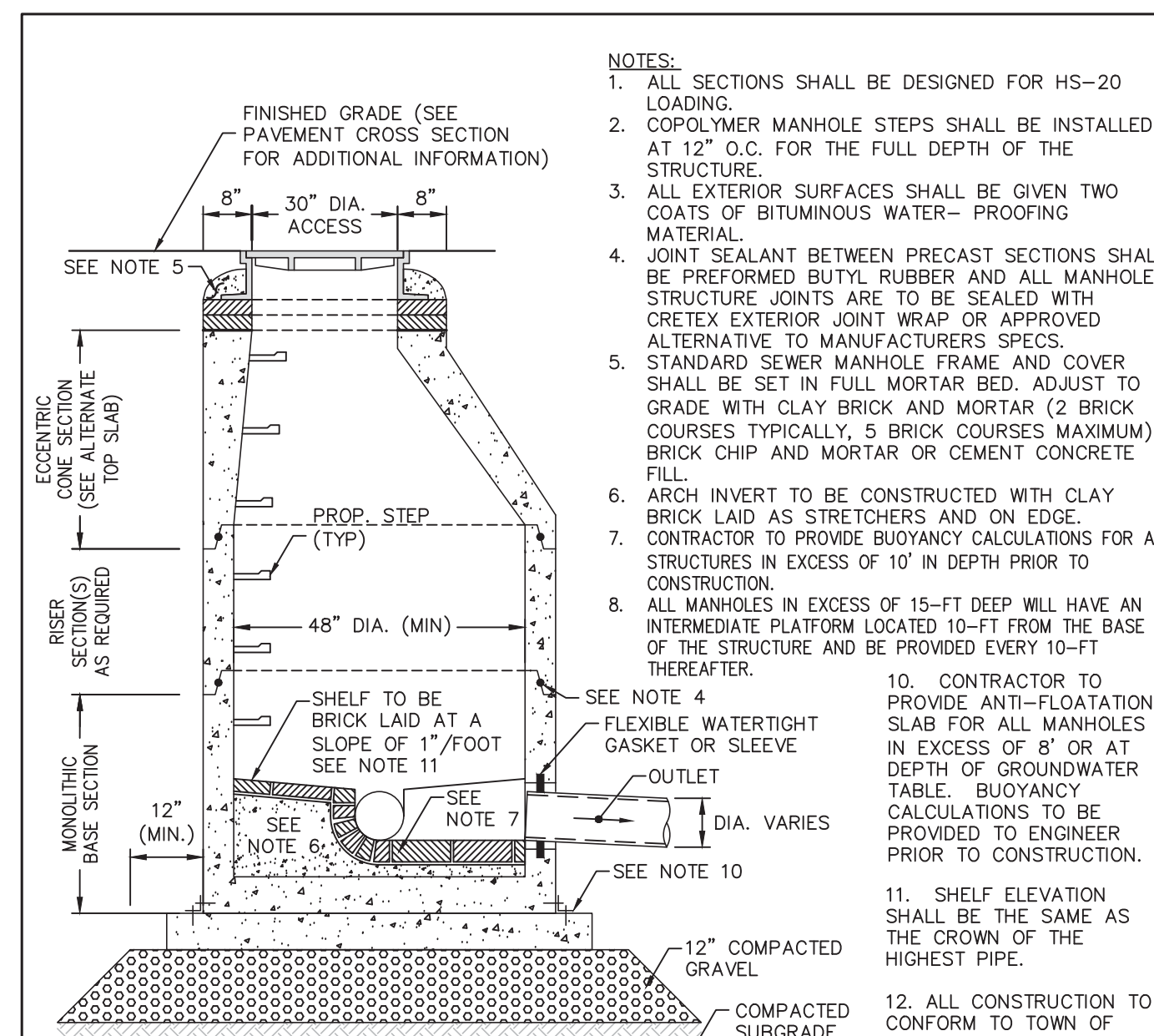
TYPICAL SANITARY SEWER MANHOLE
