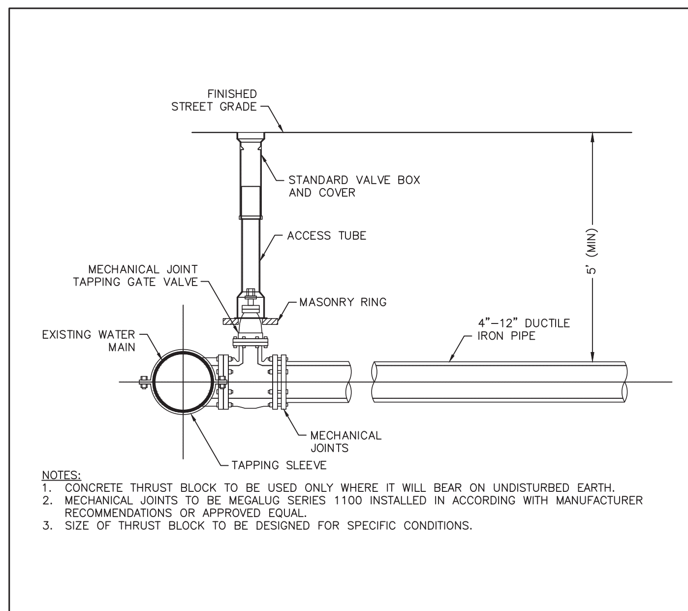
TYPICAL TAPPING SLEEVE AND VALVE DETAIL
