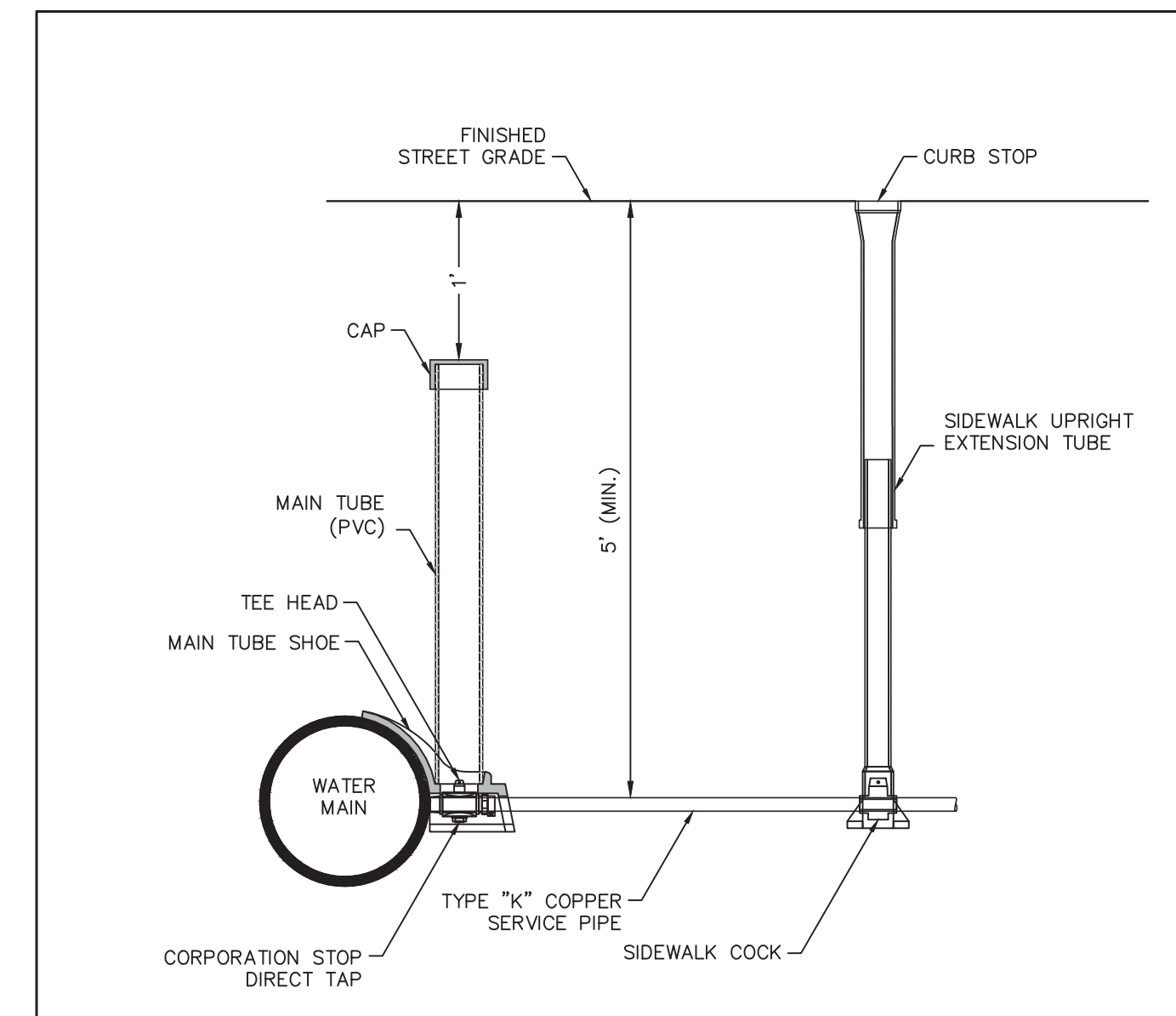
TYPICAL WATER SERVICE CONNECTION
