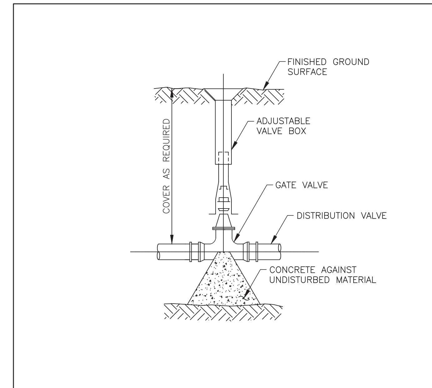
WATER GATE DETAIL
