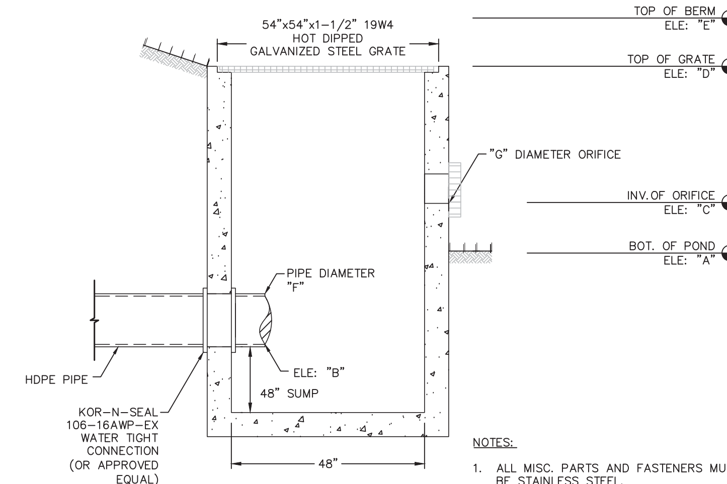
PROFILE
