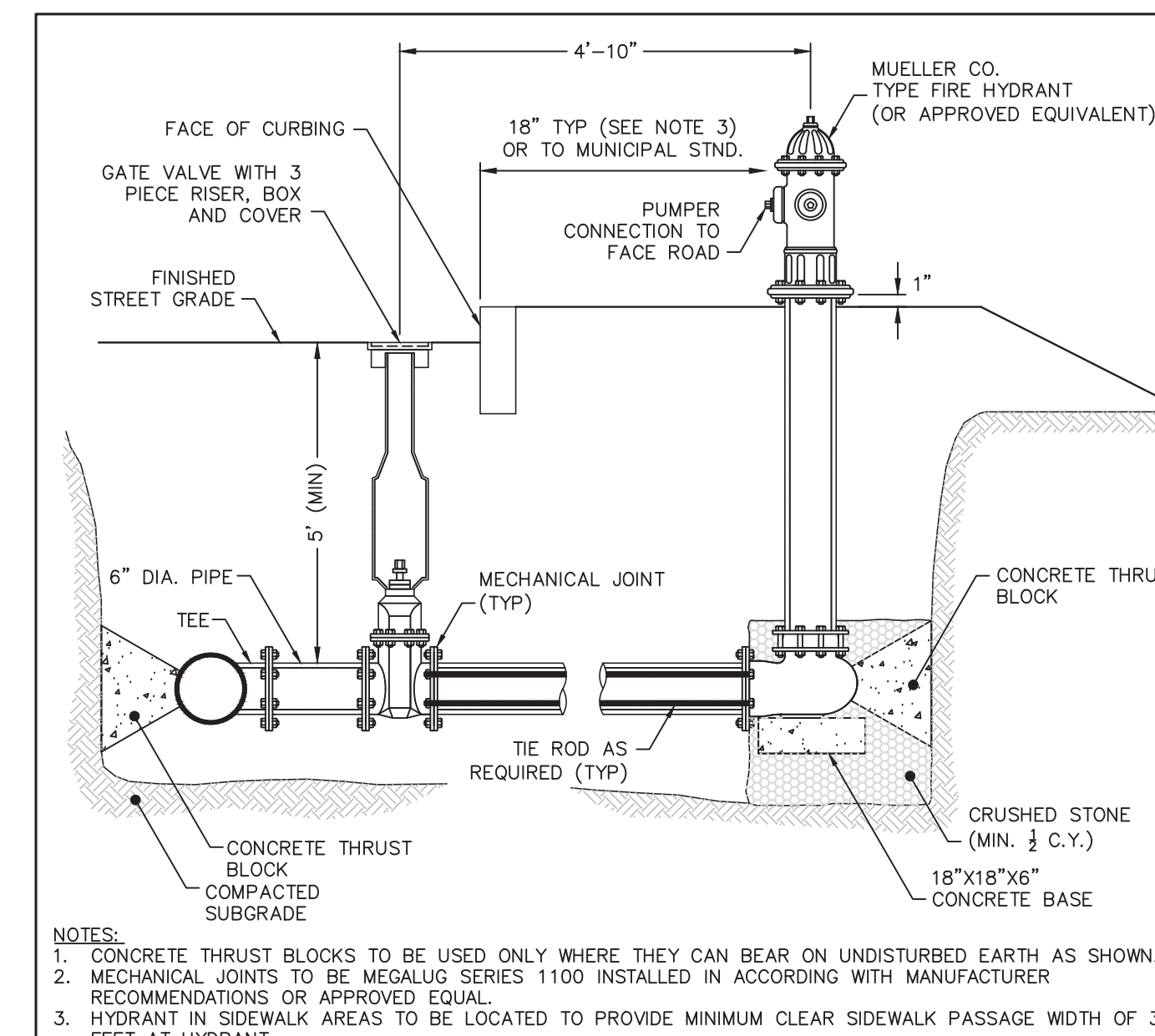
HYDRANT CONNECTION
