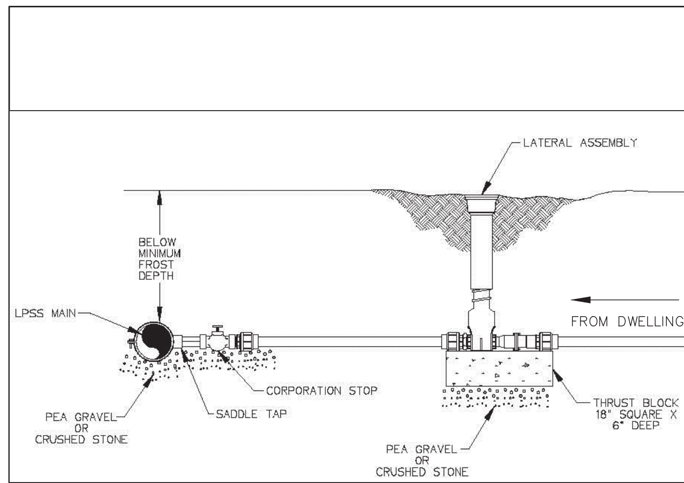
TYPICAL FLUSHING CONNECTION
