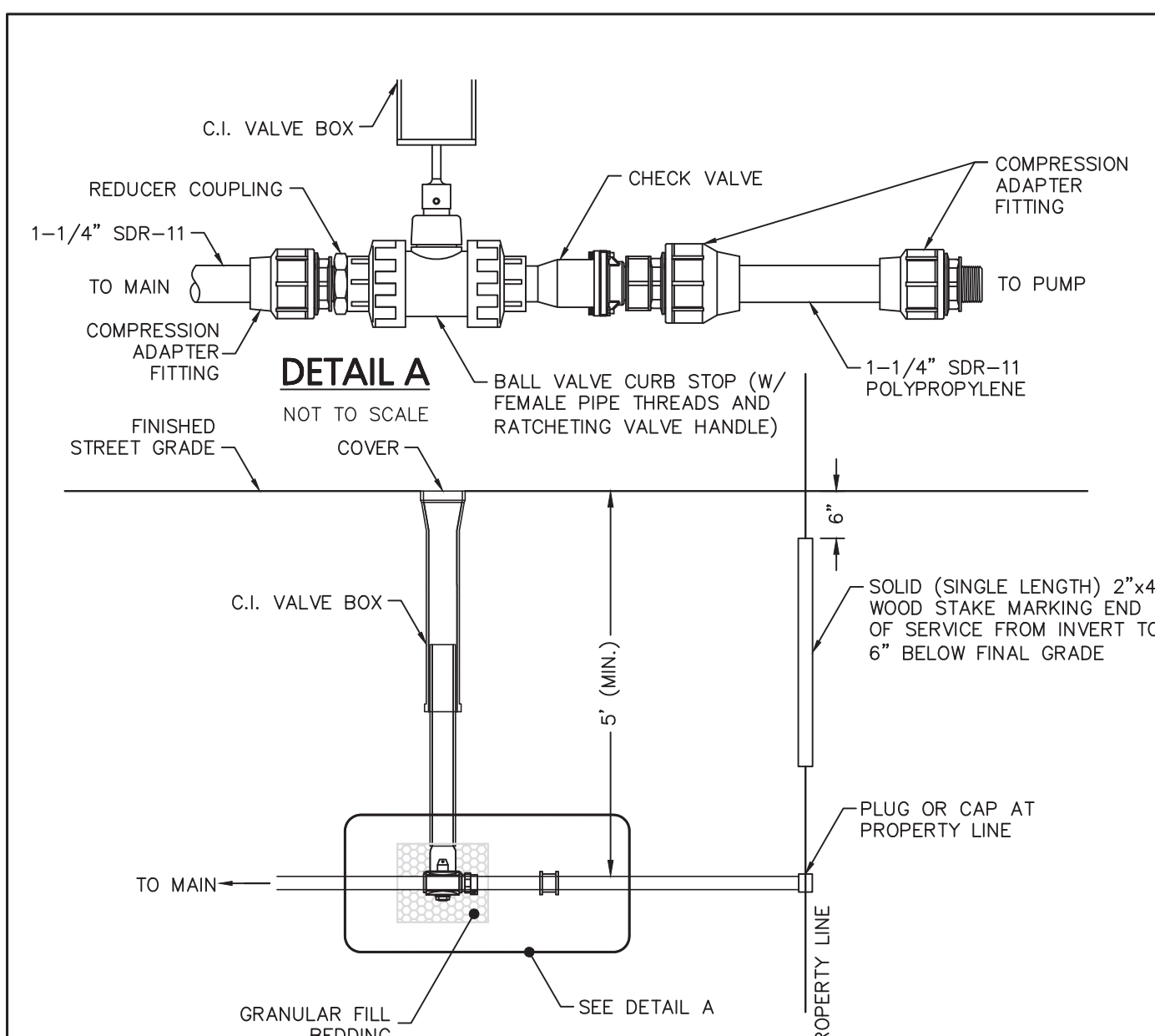
SERVICE LINE CONNECTION TO FORCE MAIN DETAIL
