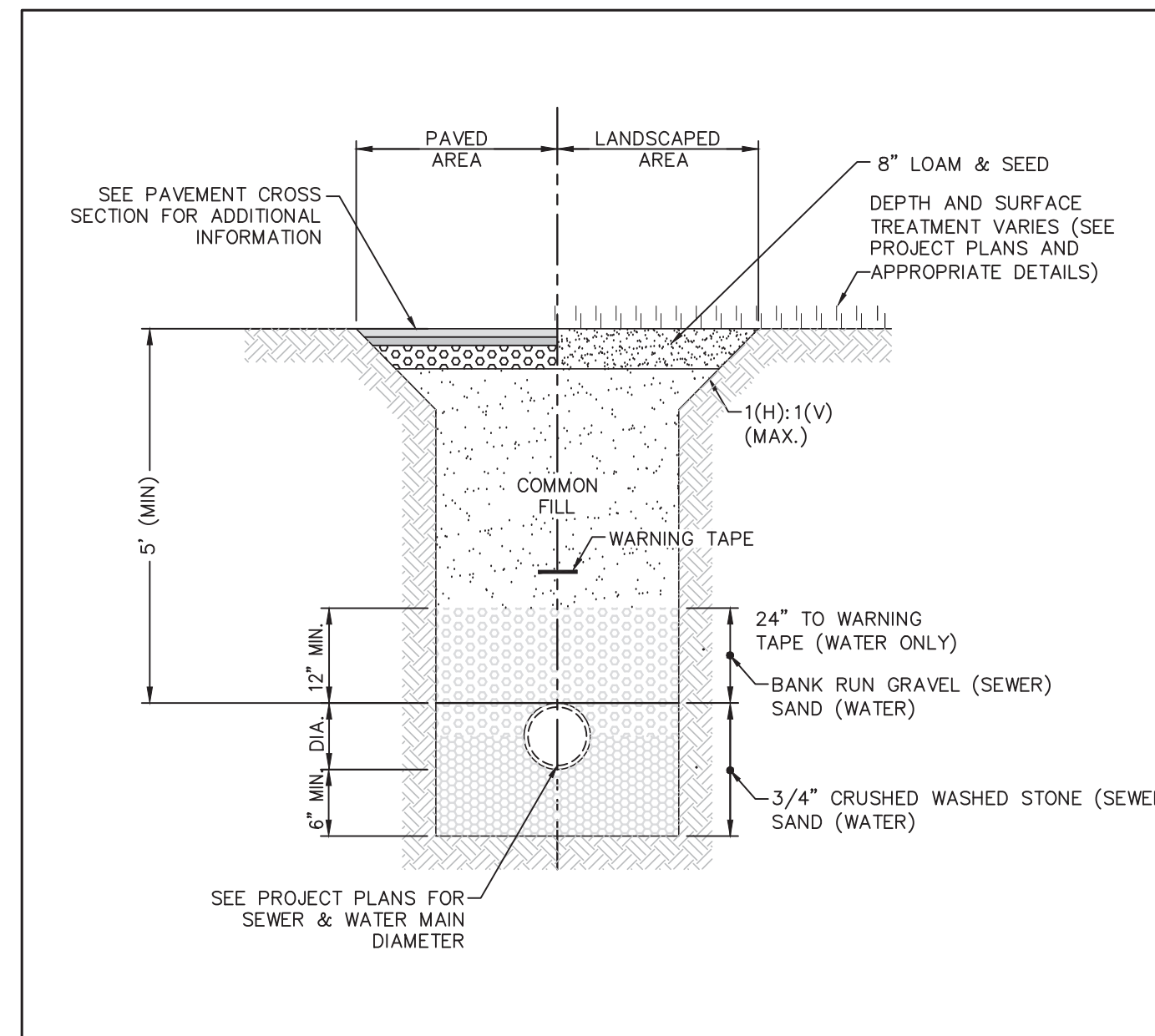
TYPICAL SEWER & WATER TRENCH
