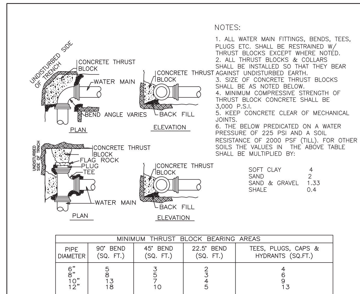
THRUST BLOCK DETAIL
