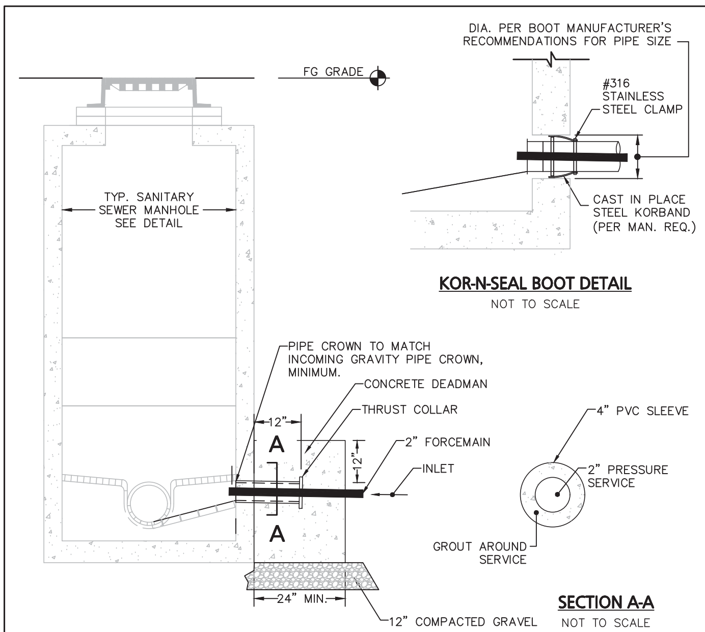
FORCE MAIN AT PROPOSED SEWER MANHOLE DETAIL
