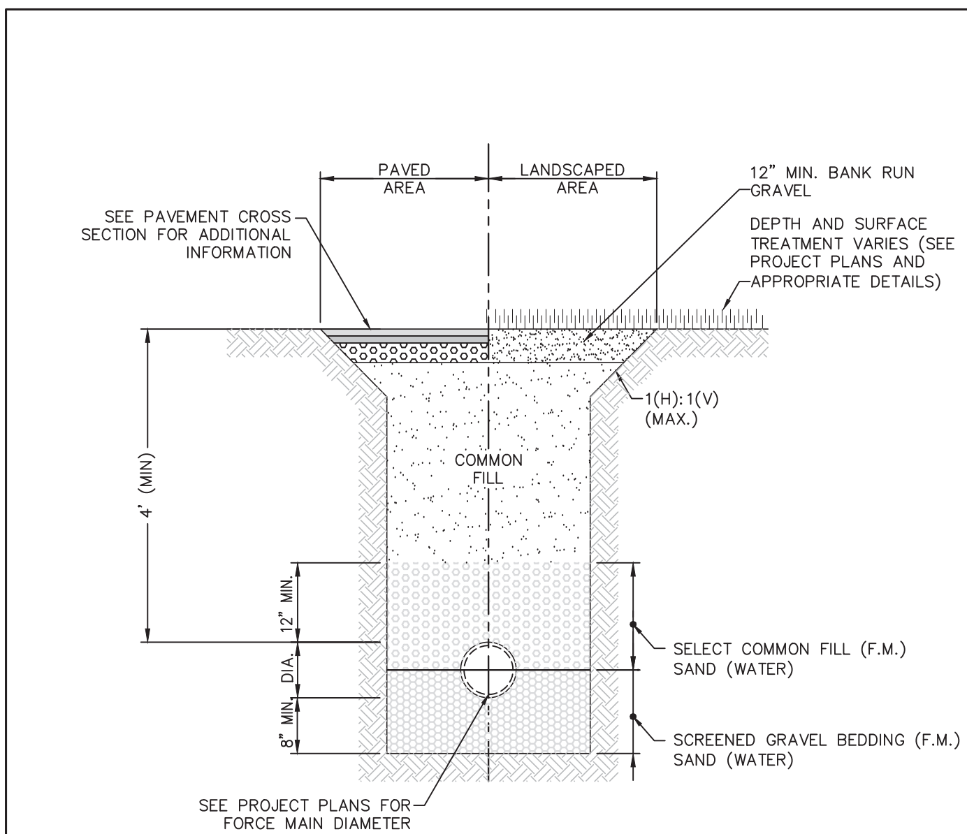
TYPICAL PRESSURE SEWER SERVICE DETAIL
