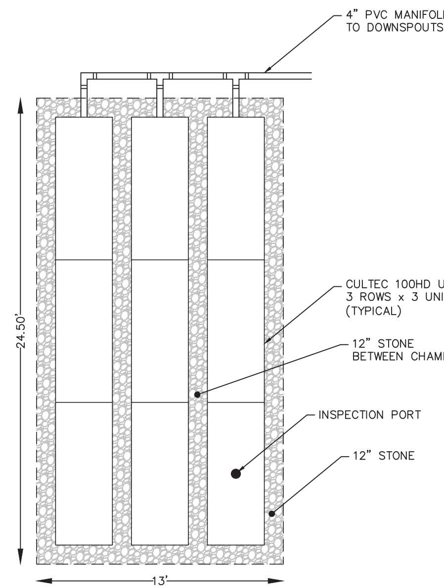
TYPICAL ROOF DRYWELL
