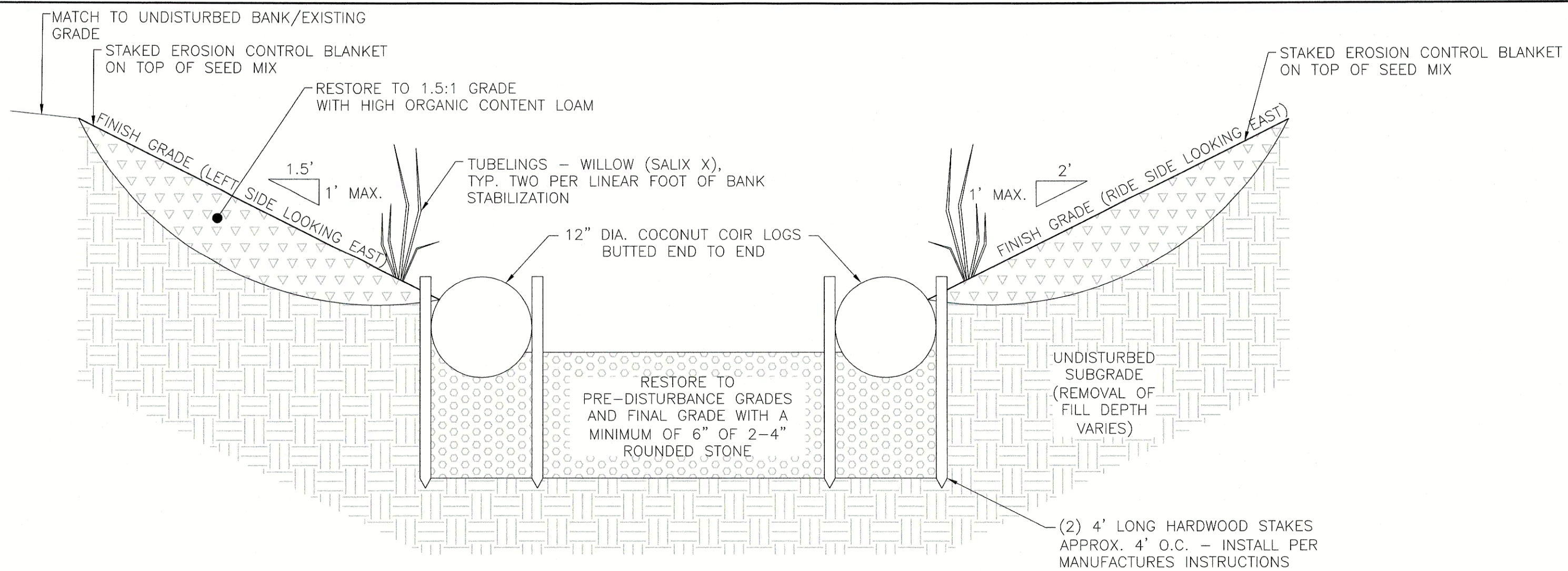
BANK STABILIZATION WITH COCONUT COIR LOGS AND TUBELINGS DETAIL (NOT TO SCALE)
