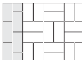
4" x 8" Double Sailor Course w/ Basket Weave Pattern
