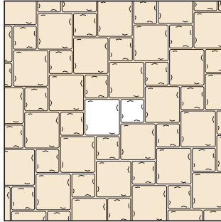
GS Pattern 1 69 sf Grand Squares 31 sf Squares
